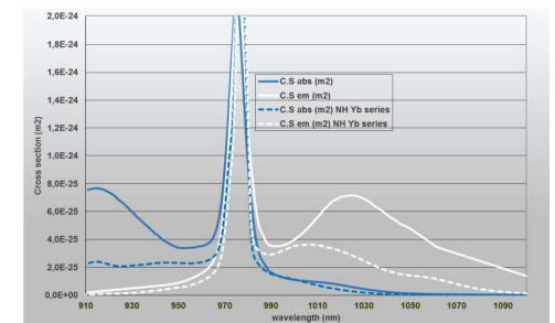
Yb Double Clad Cross section files
