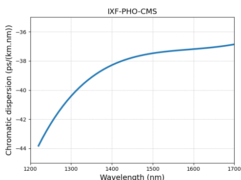
Typical dispersion profile of the IXF-PHO-CMS fiber
